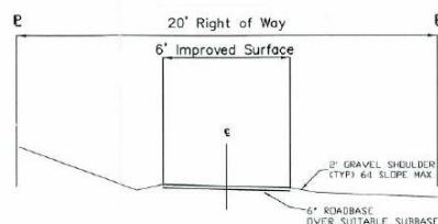
PROPOSED 6' TRAIL
