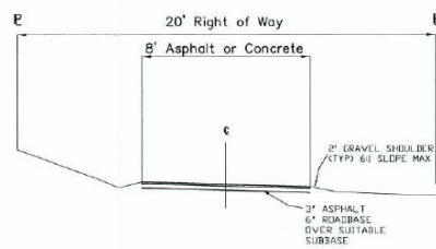
PROPOSED 8' TRAIL
